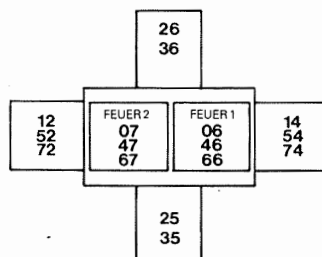
JOYSTICK 1
