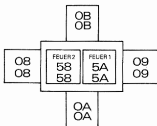
JOYSTICK 0
